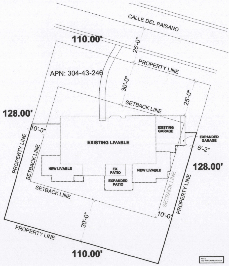
SITE PLAN 1" = 10'-0"
